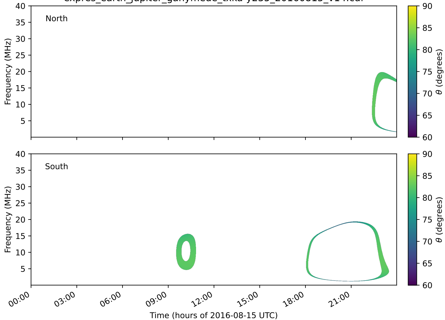
expres_earth_jupiter_ganymede_txka-y235_20160815_v14.cdf
