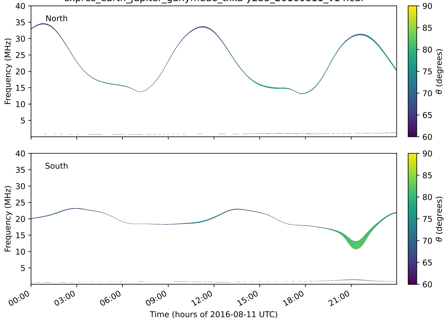
expres_earth_jupiter_ganymede_txka-y235_20160811_v14.cdf
