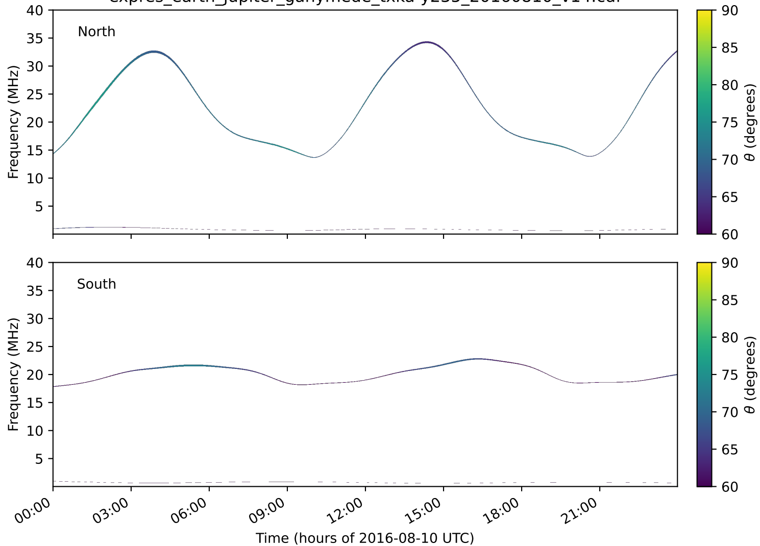
expres_earth_jupiter_ganymede_txka-y235_20160810_v14.cdf
