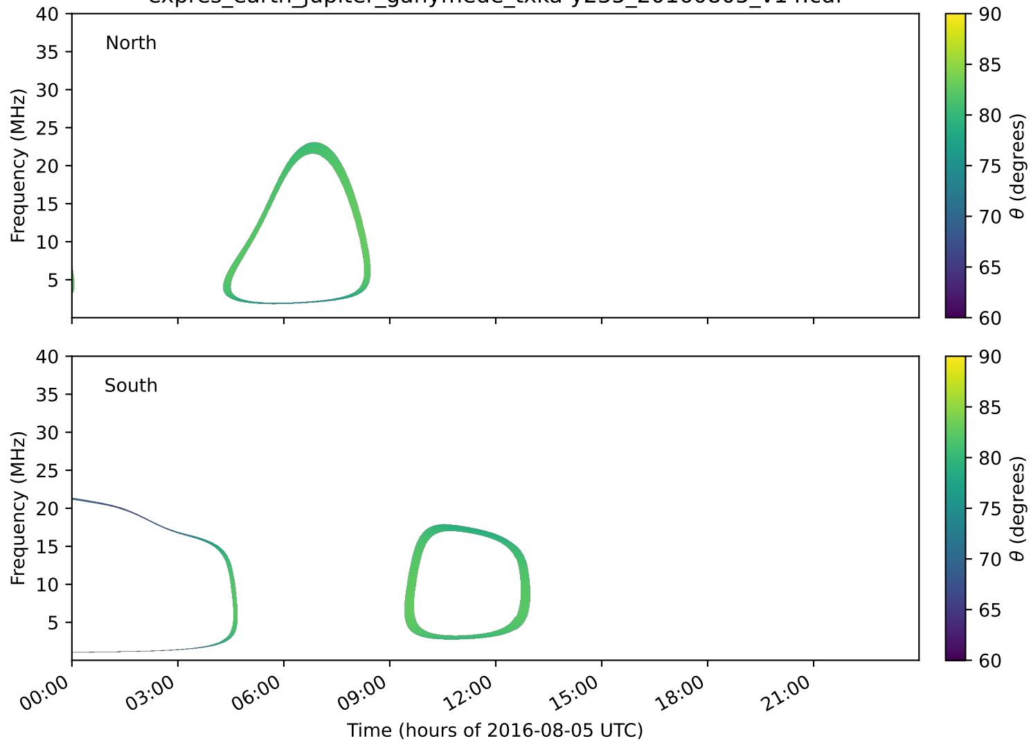
expres_earth_jupiter_ganymede_txka-y235_20160805_v14.cdf
