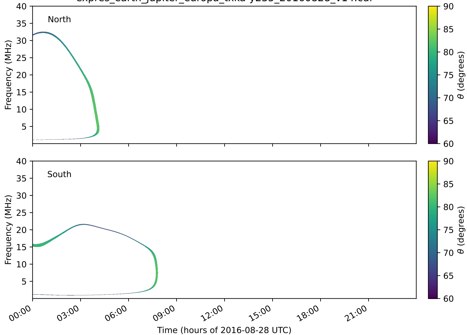
expres_earth_jupiter_europa_txka-y235_20160828_v14.cdf
