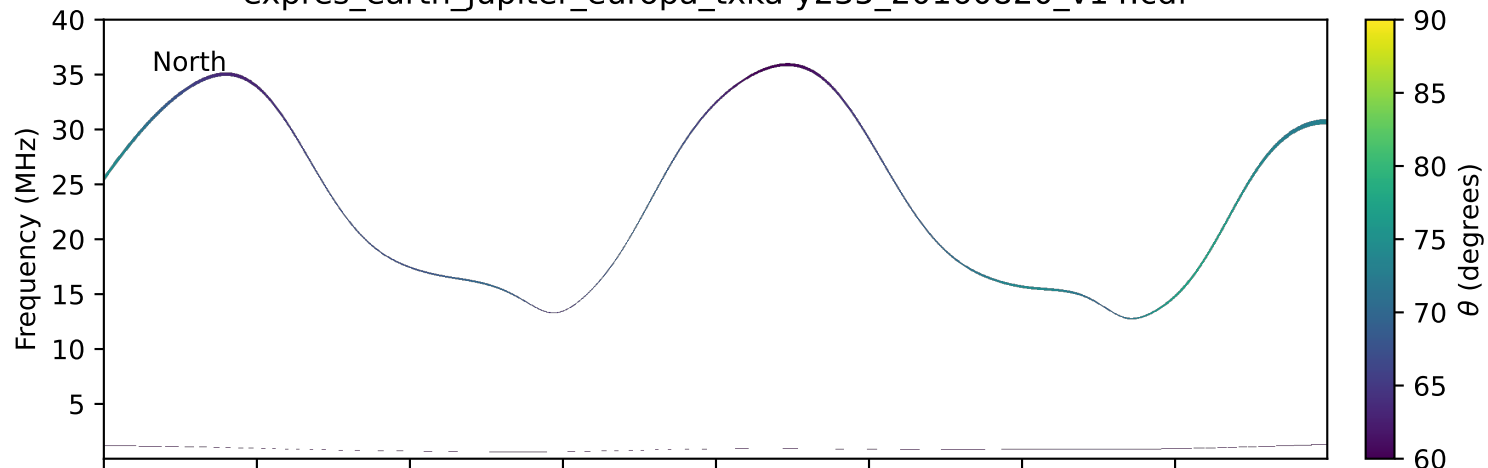
expres_earth_jupiter_europa_txka-y235_20160820_v14.cdf
