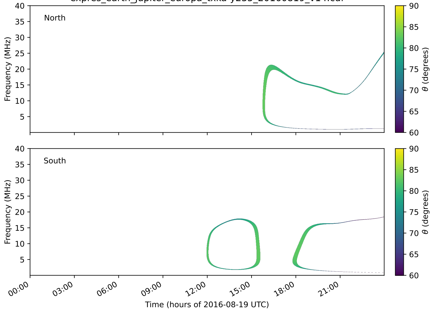
expres_earth_jupiter_europa_txka-y235_20160819_v14.cdf
