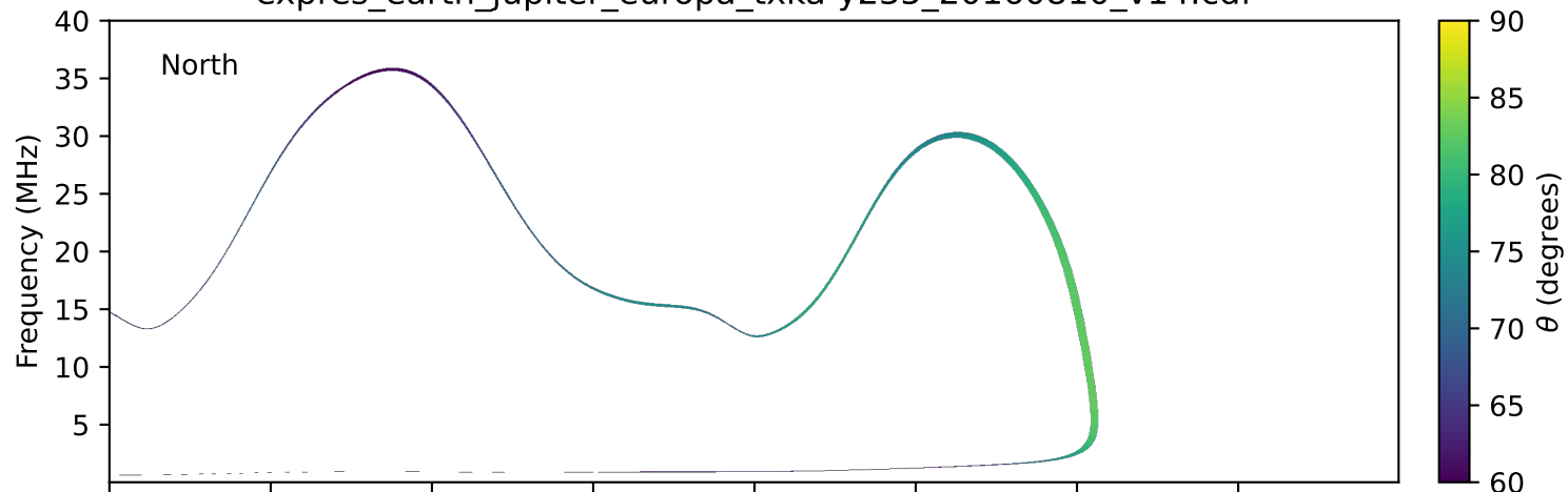
expres_earth_jupiter_europa_txka-y235_20160810_v14.cdf
