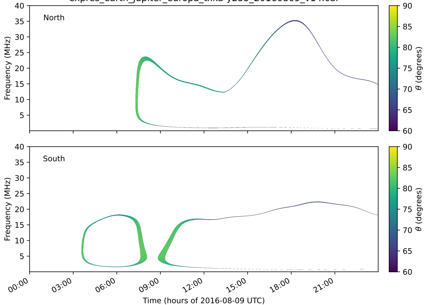
expres_earth_jupiter_europa_txka-y235_20160809_v14.cdf
