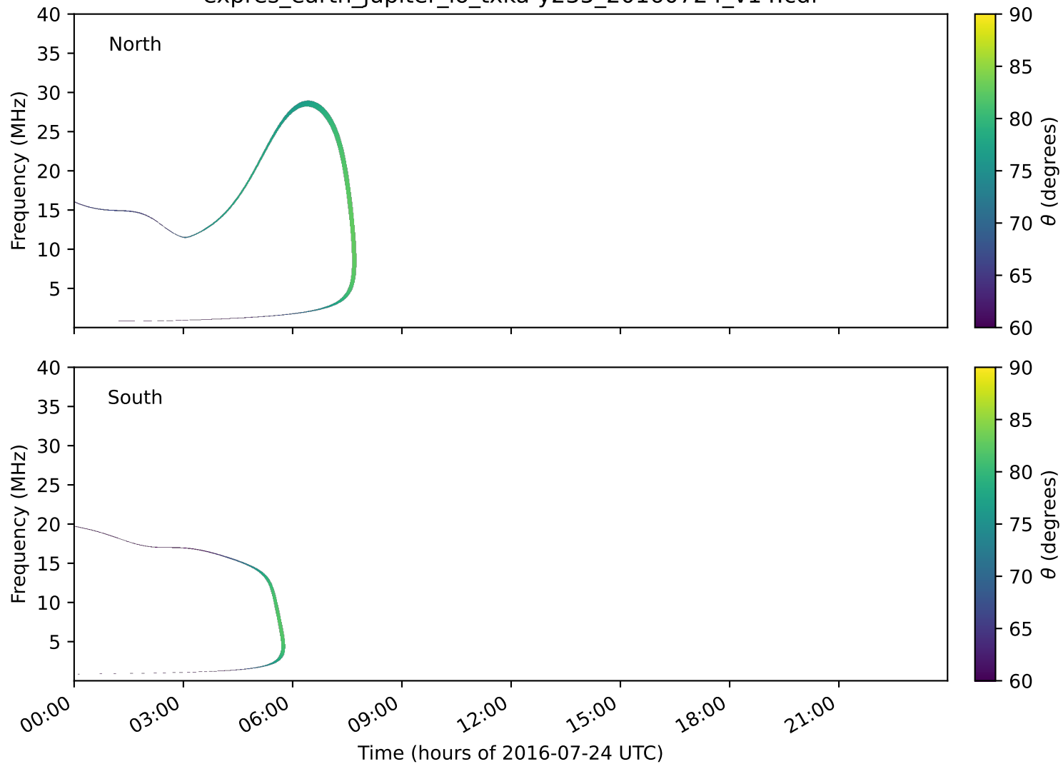
expres_earth_jupiter_io_txka-y235_20160724_v14.cdf
