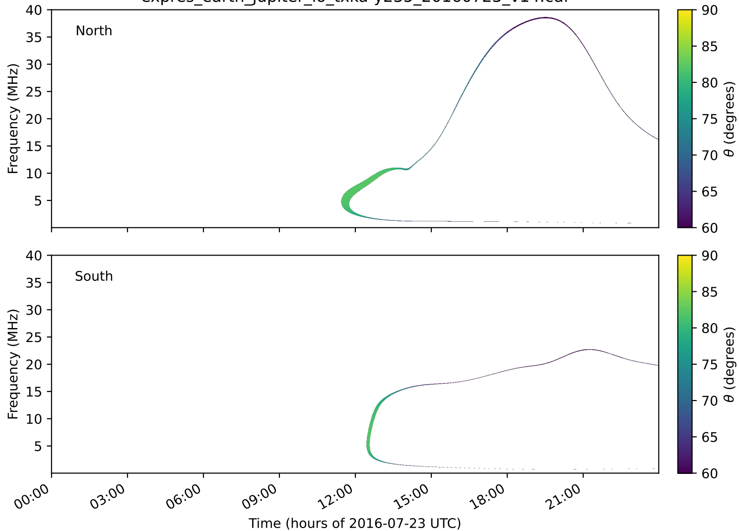
expres_earth_jupiter_io_txka-y235_20160723_v14.cdf
