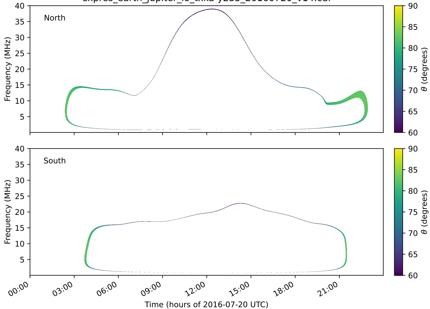
expres_earth_jupiter_io_txka-y235_20160720_v14.cdf
