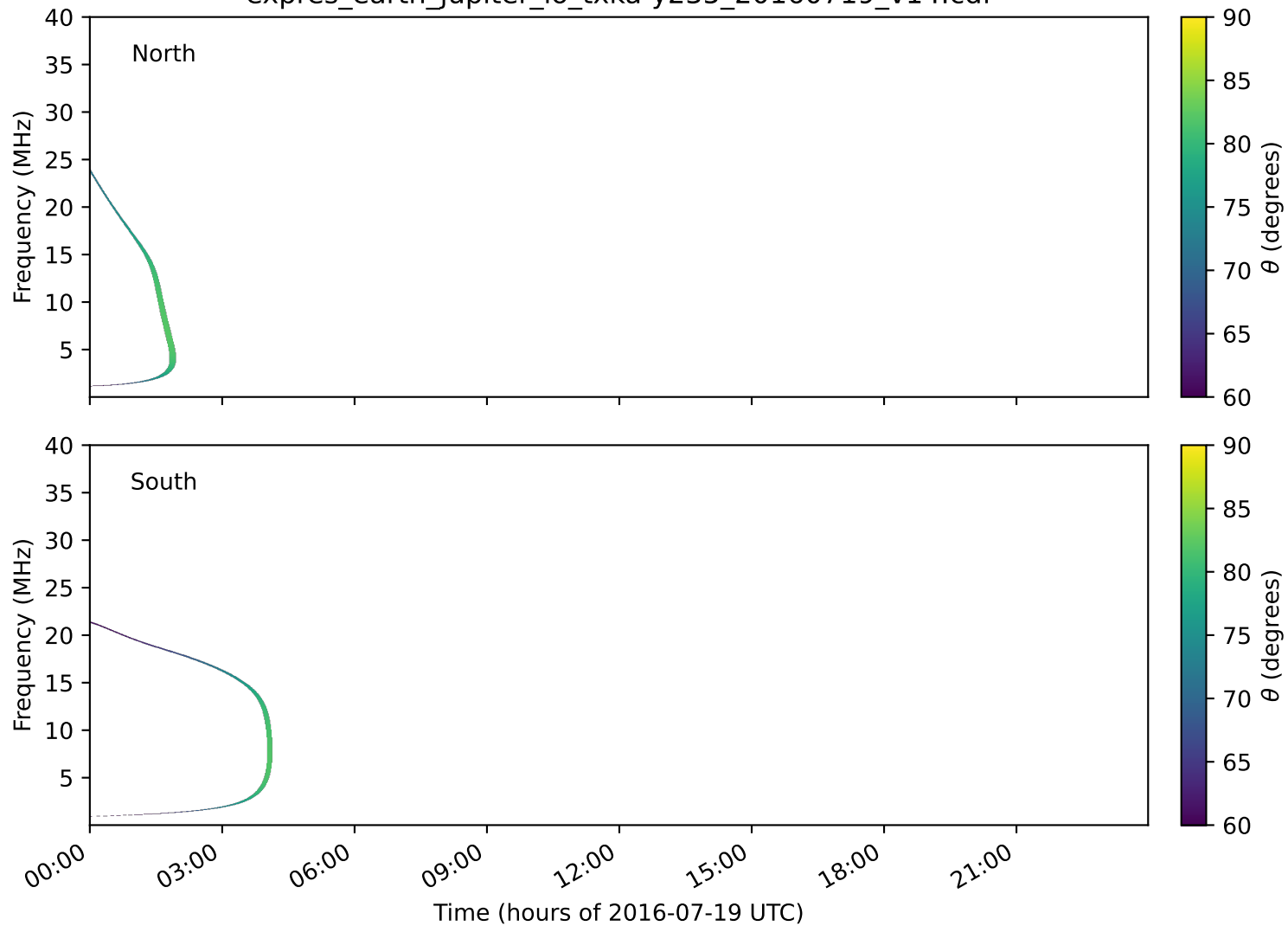
expres_earth_jupiter_io_txka-y235_20160719_v14.cdf
