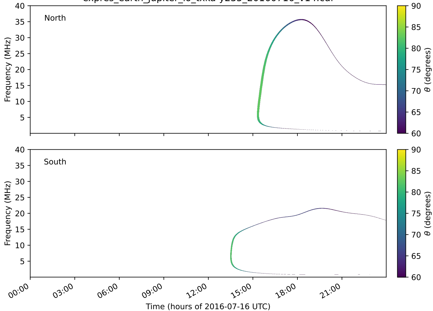
expres_earth_jupiter_io_txka-y235_20160716_v14.cdf
