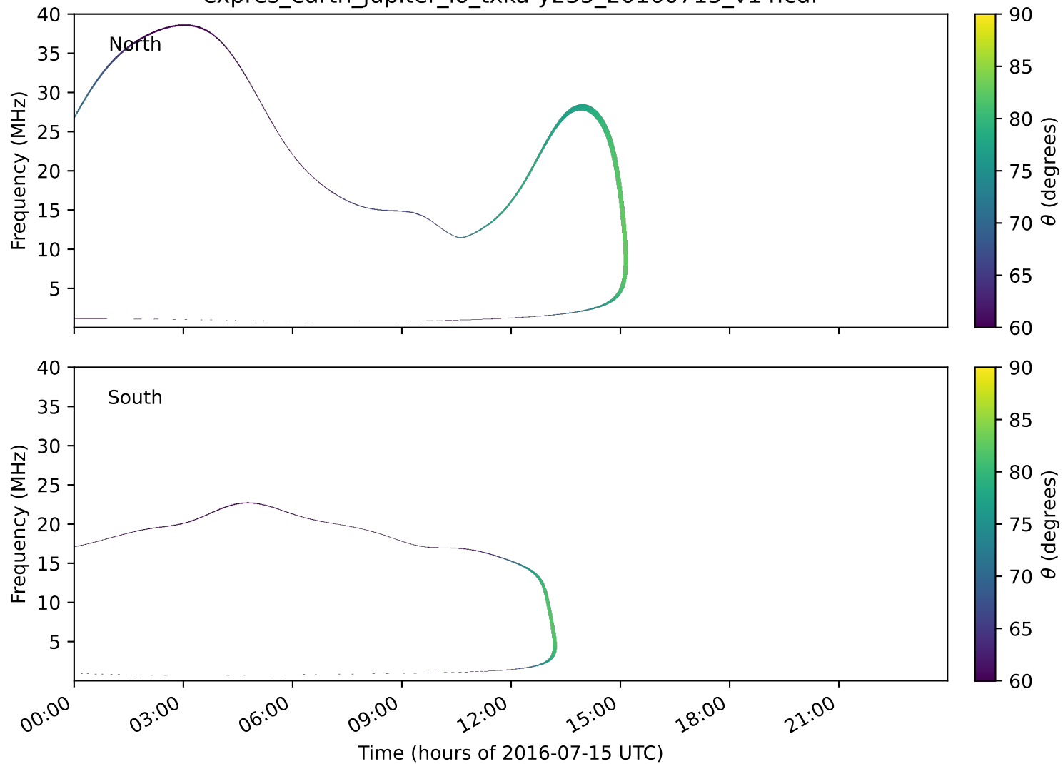
expres_earth_jupiter_io_txka-y235_20160715_v14.cdf
