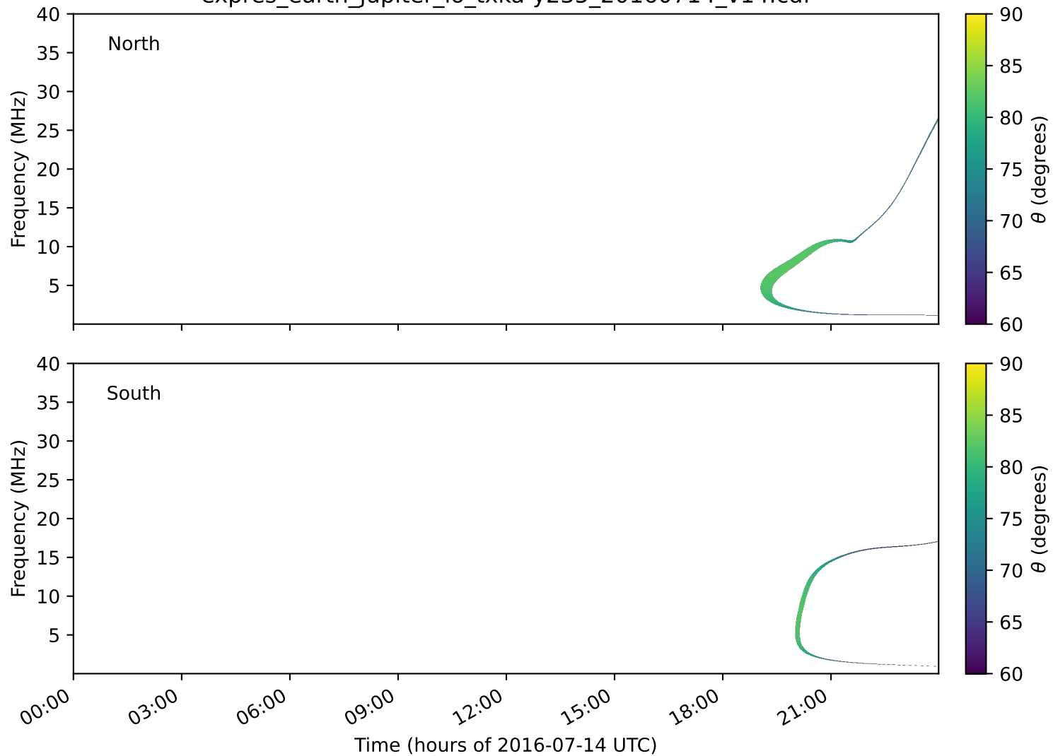
expres_earth_jupiter_io_txka-y235_20160714_v14.cdf
