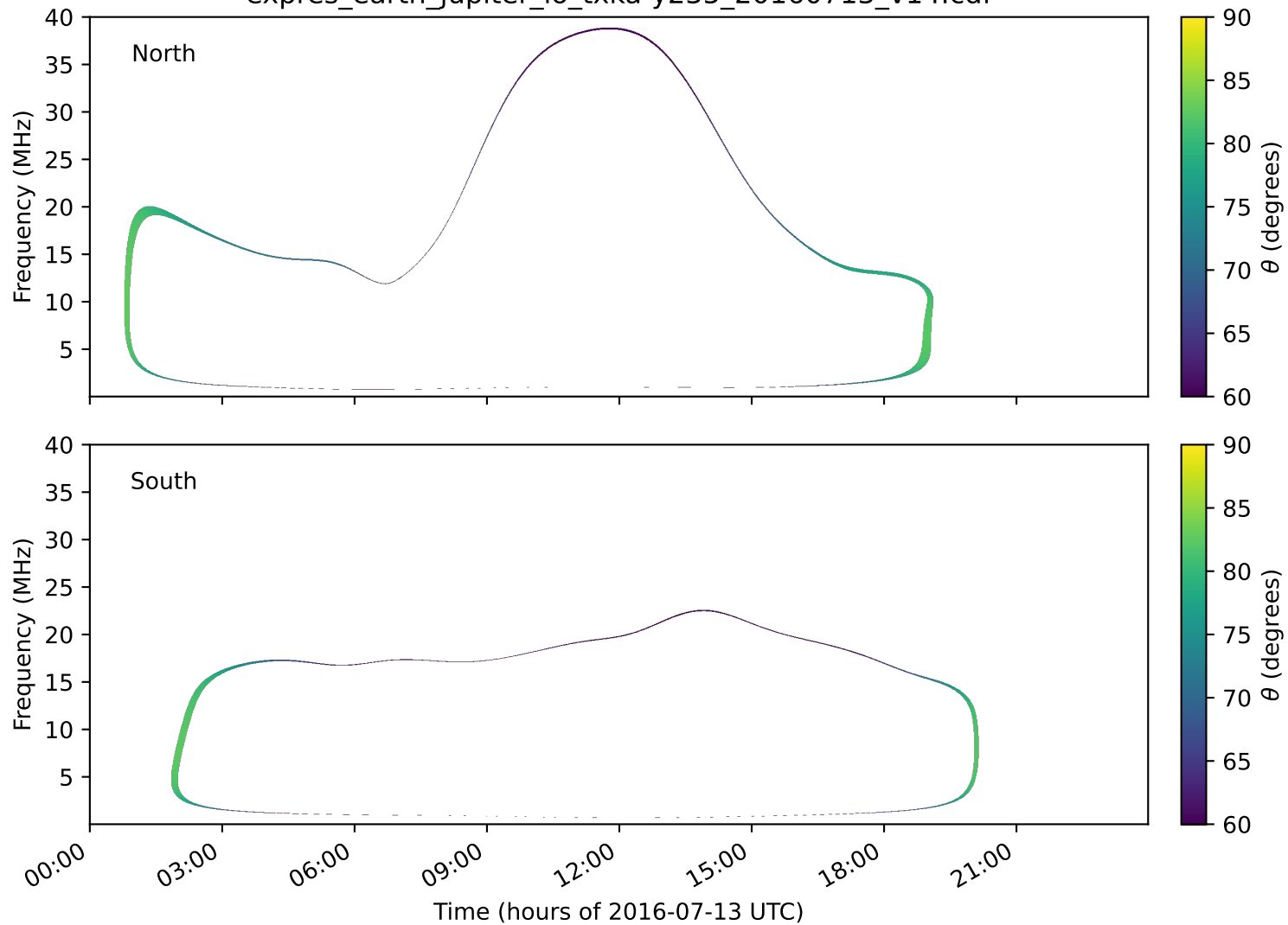
expres_earth_jupiter_io_txka-y235_20160713_v14.cdf
