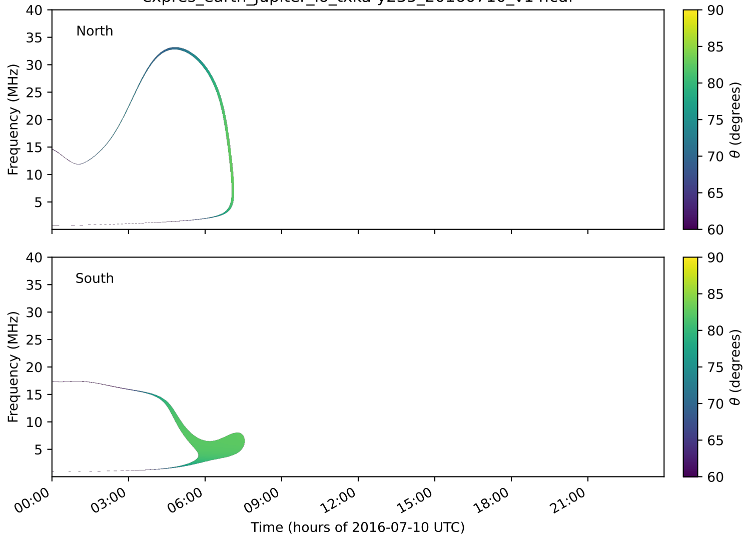
expres_earth_jupiter_io_txka-y235_20160710_v14.cdf
