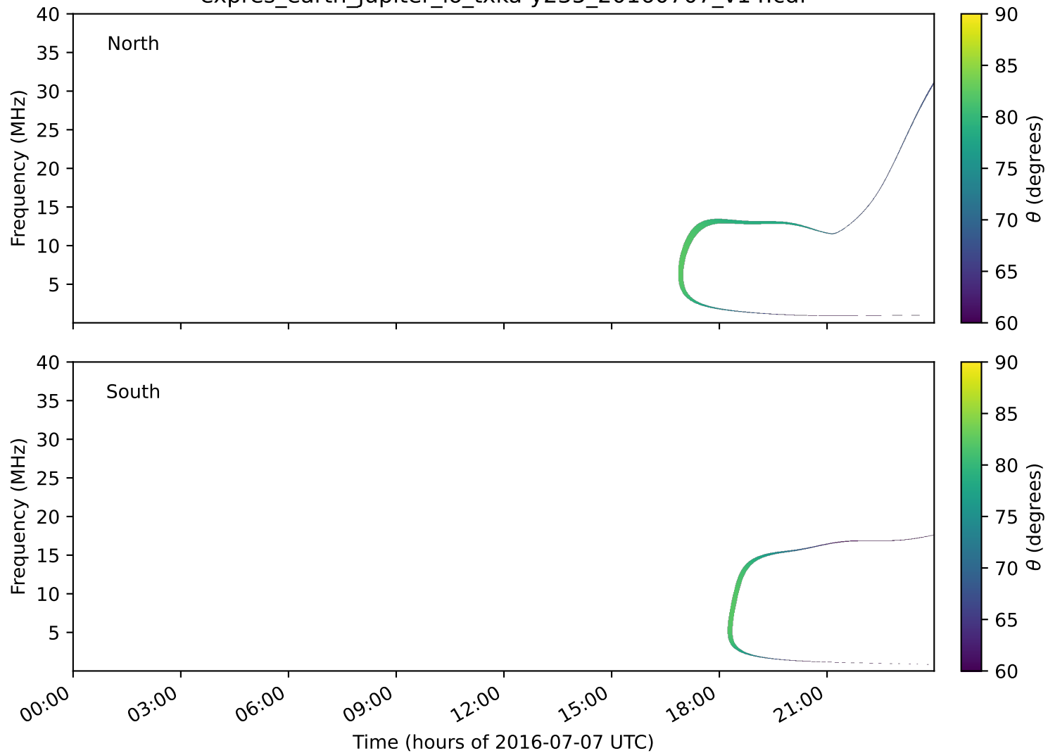
expres_earth_jupiter_io_txka-y235_20160707_v14.cdf
