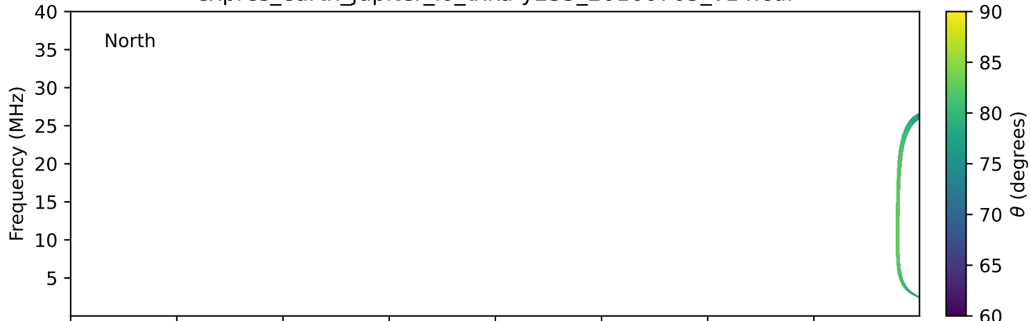
expres_earth_jupiter_io_txka-y235_20160705_v14.cdf
