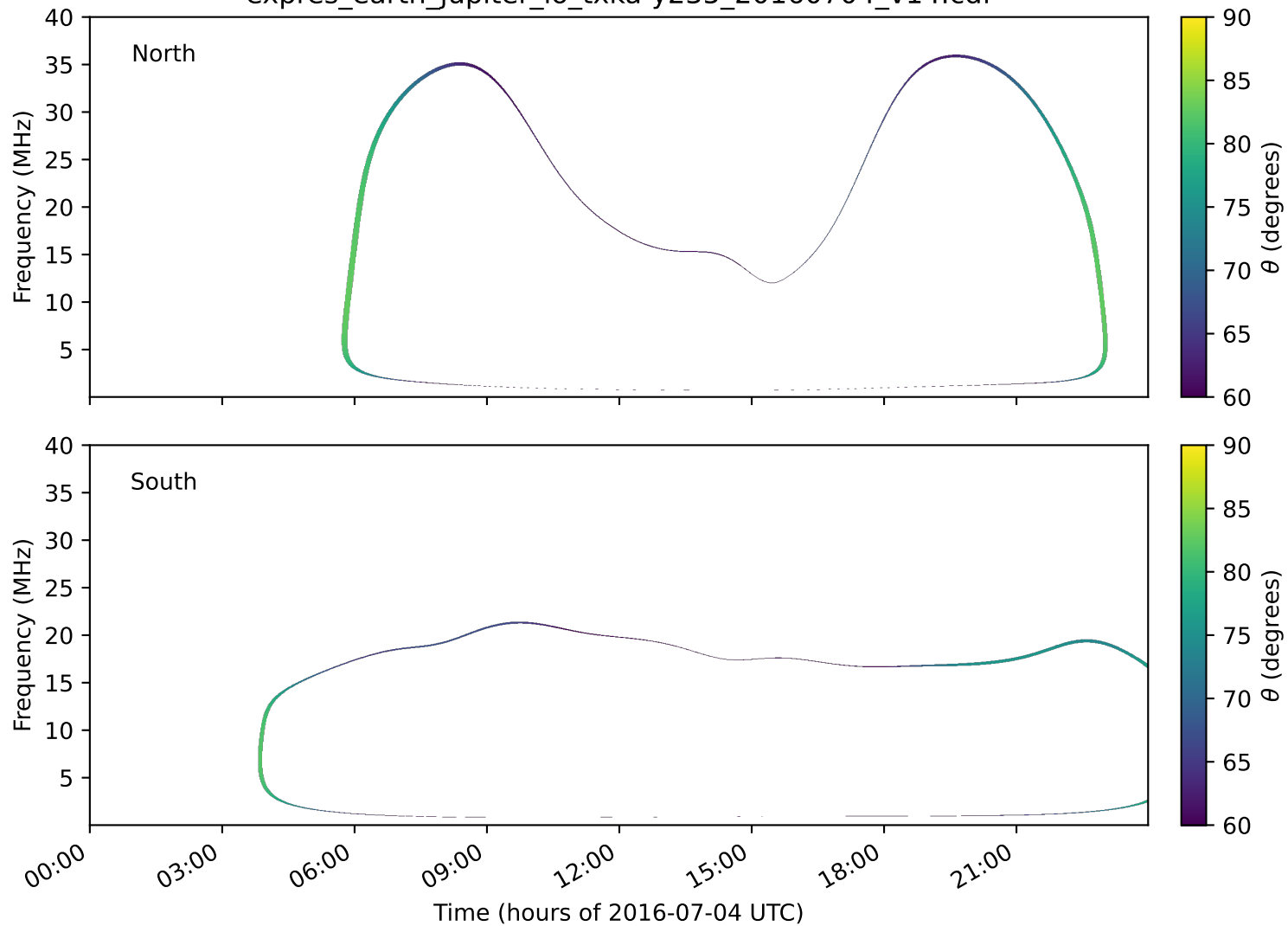
expres_earth_jupiter_io_txka-y235_20160704_v14.cdf
