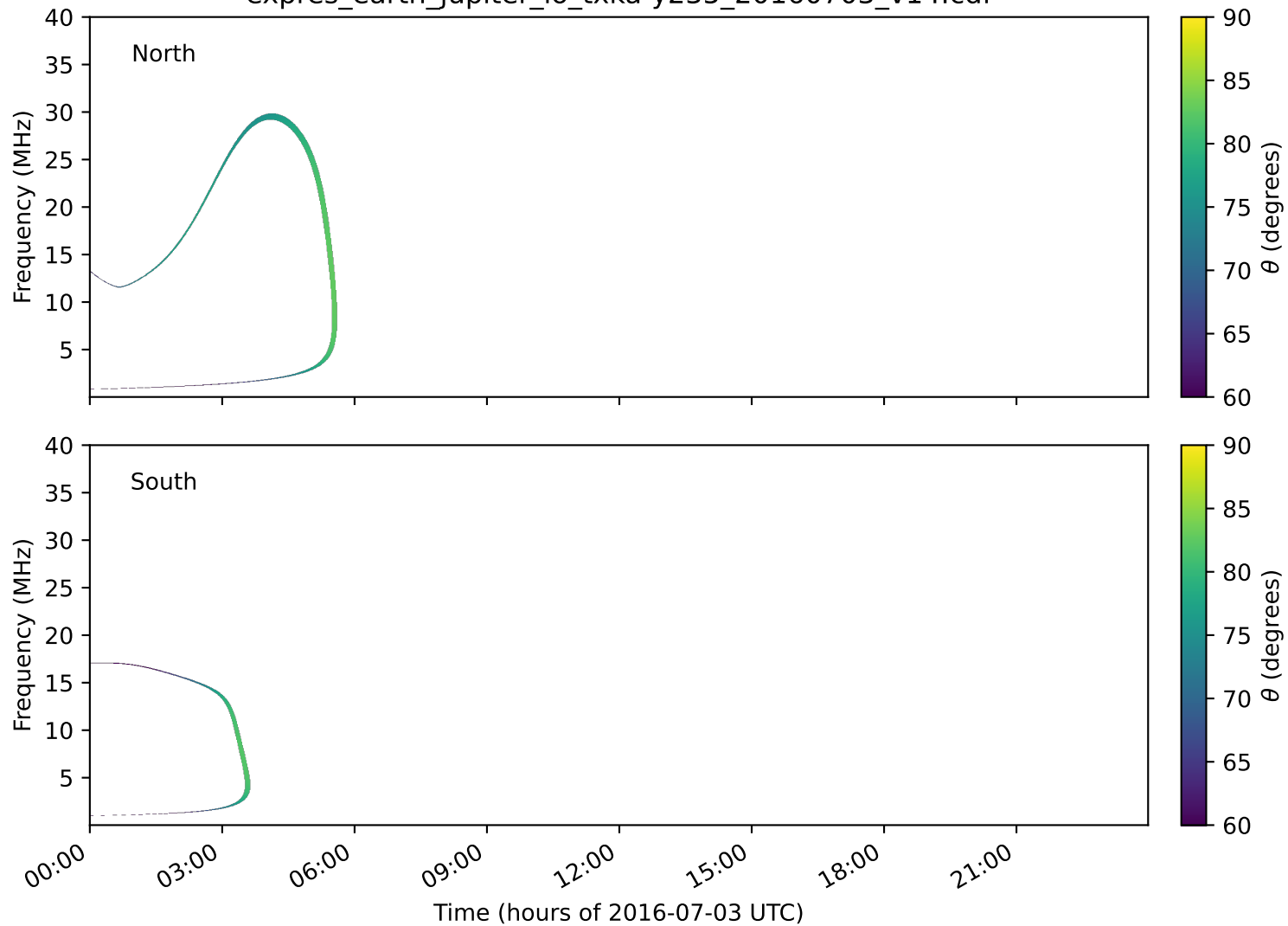
expres_earth_jupiter_io_txka-y235_20160703_v14.cdf
