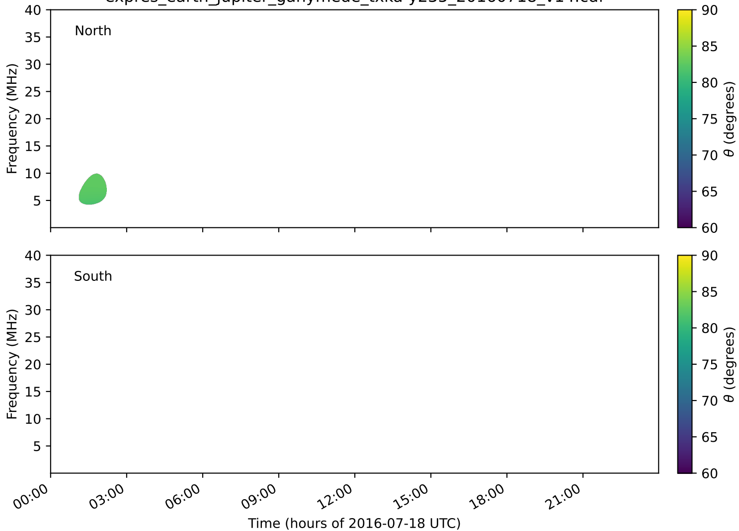
expres_earth_jupiter_ganymede_txka-y235_20160718_v14.cdf
