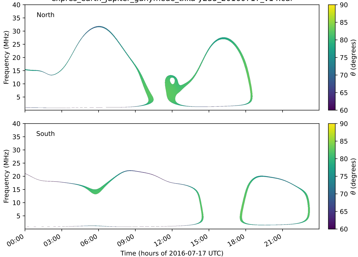
expres_earth_jupiter_ganymede_txka-y235_20160717_v14.cdf
