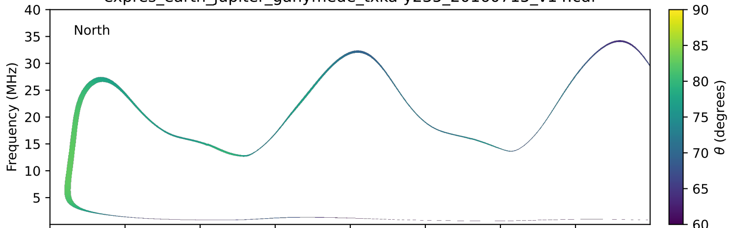
expres_earth_jupiter_ganymede_txka-y235_20160715_v14.cdf
