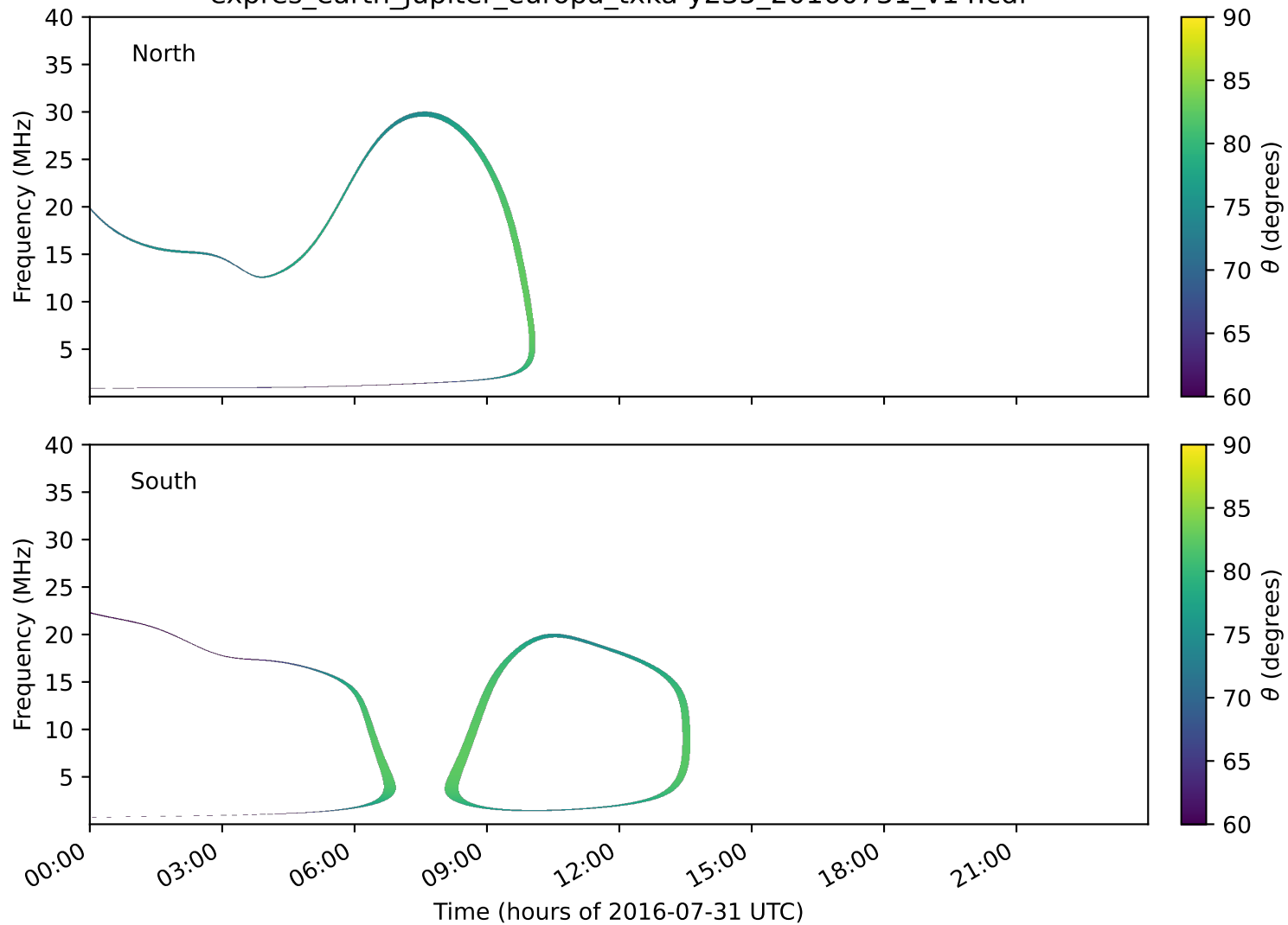
expres_earth_jupiter_europa_txka-y235_20160731_v14.cdf
