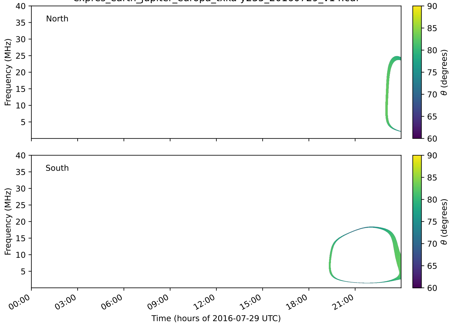
expres_earth_jupiter_europa_txka-y235_20160729_v14.cdf
