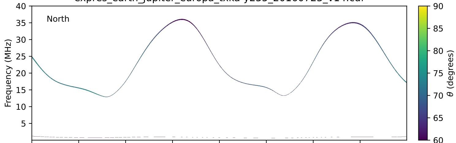
expres_earth_jupiter_europa_txka-y235_20160723_v14.cdf
