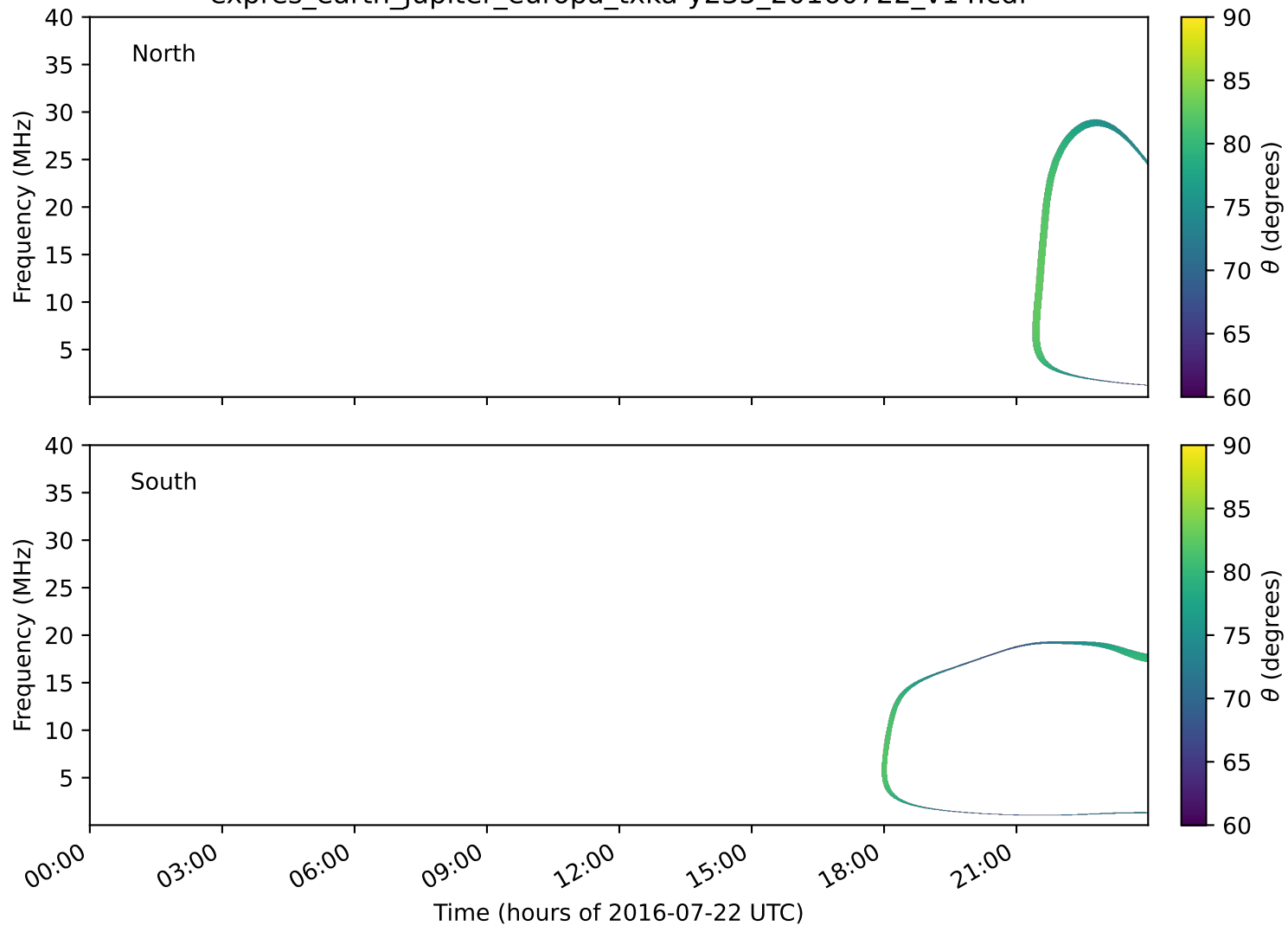
expres_earth_jupiter_europa_txka-y235_20160722_v14.cdf
