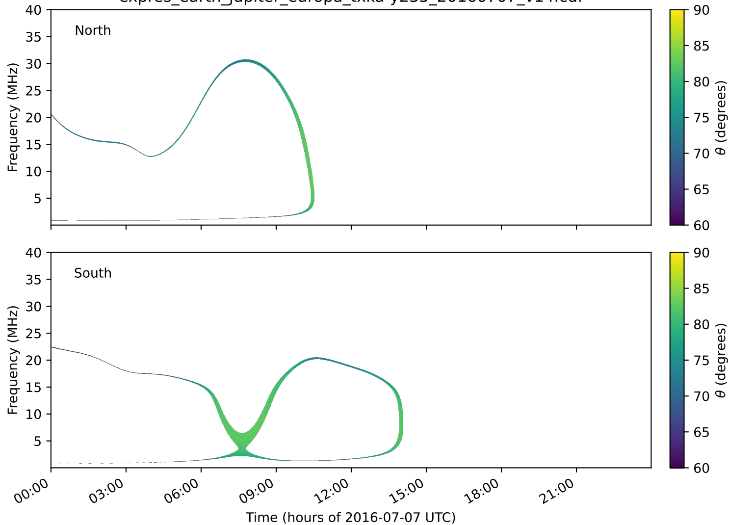
expres_earth_jupiter_europa_txka-y235_20160707_v14.cdf
