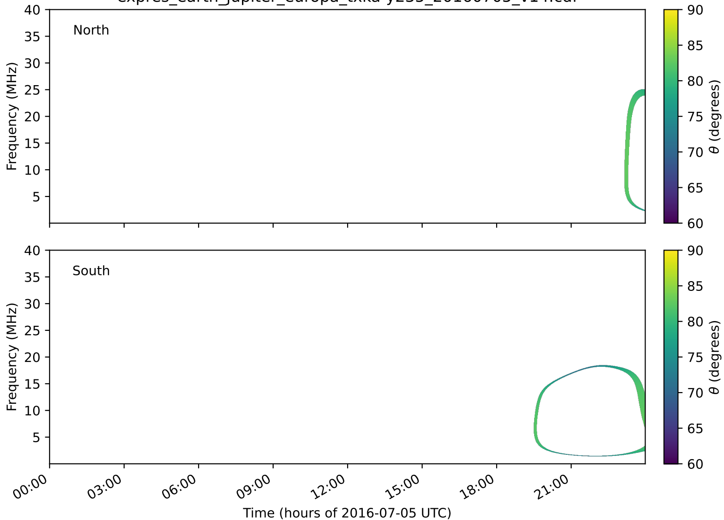
expres_earth_jupiter_europa_txka-y235_20160705_v14.cdf
