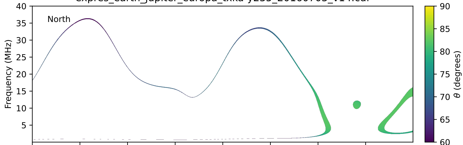
expres_earth_jupiter_europa_txka-y235_20160703_v14.cdf
