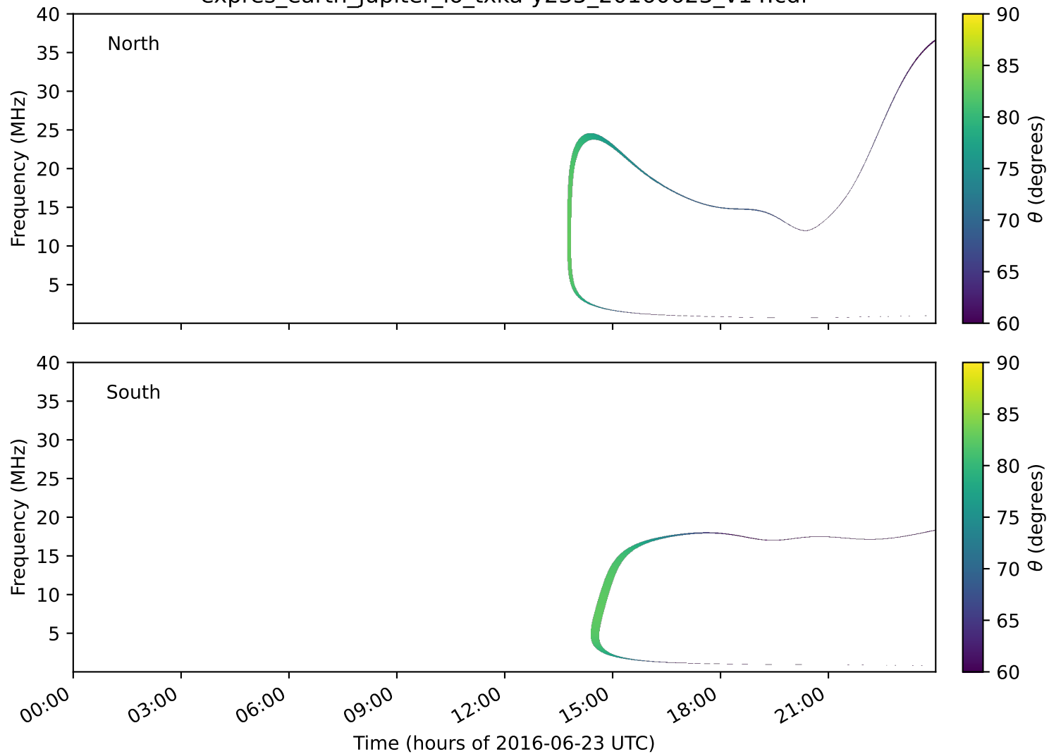
expres_earth_jupiter_io_txka-y235_20160623_v14.cdf
