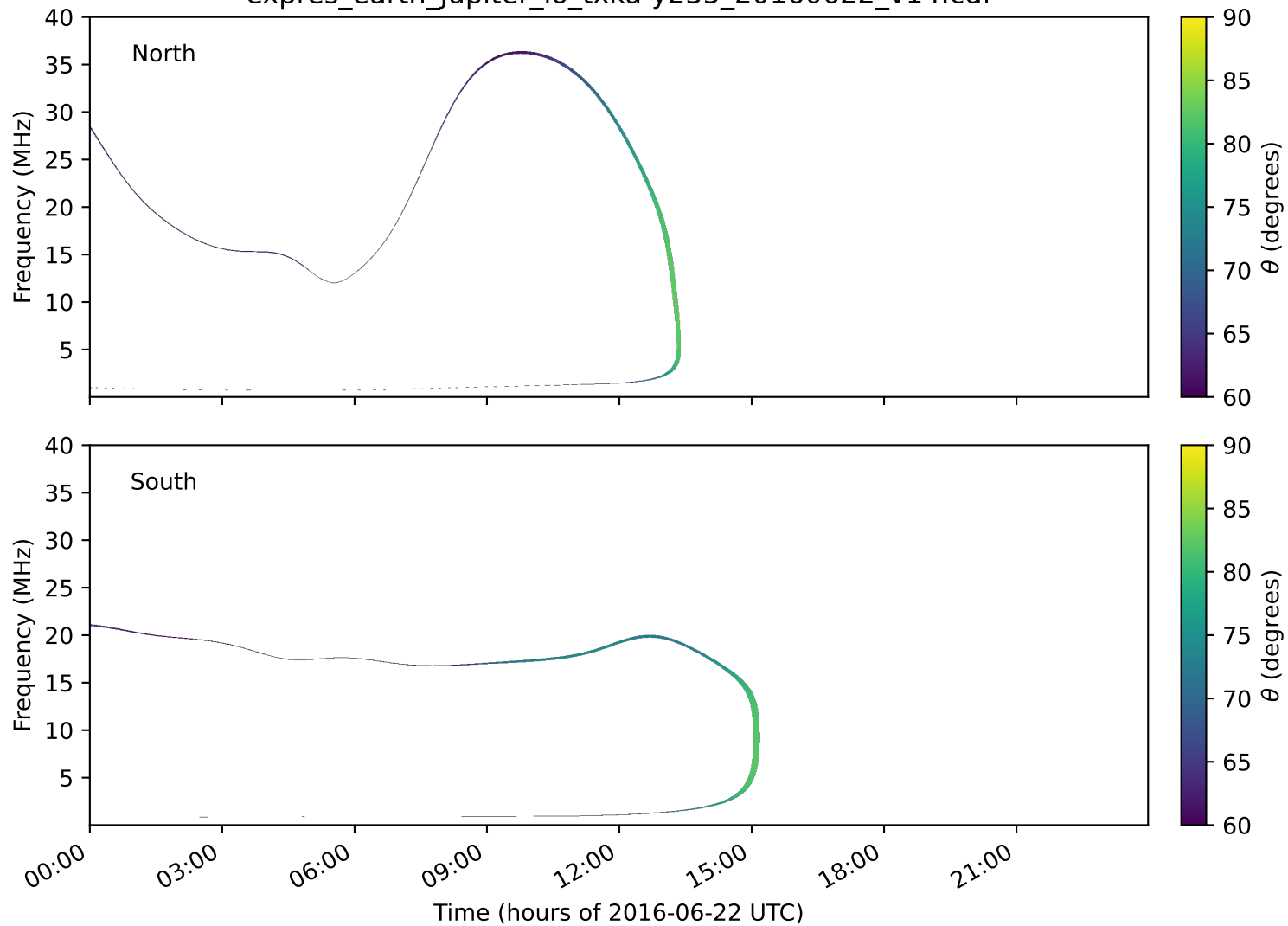
expres_earth_jupiter_io_txka-y235_20160622_v14.cdf
