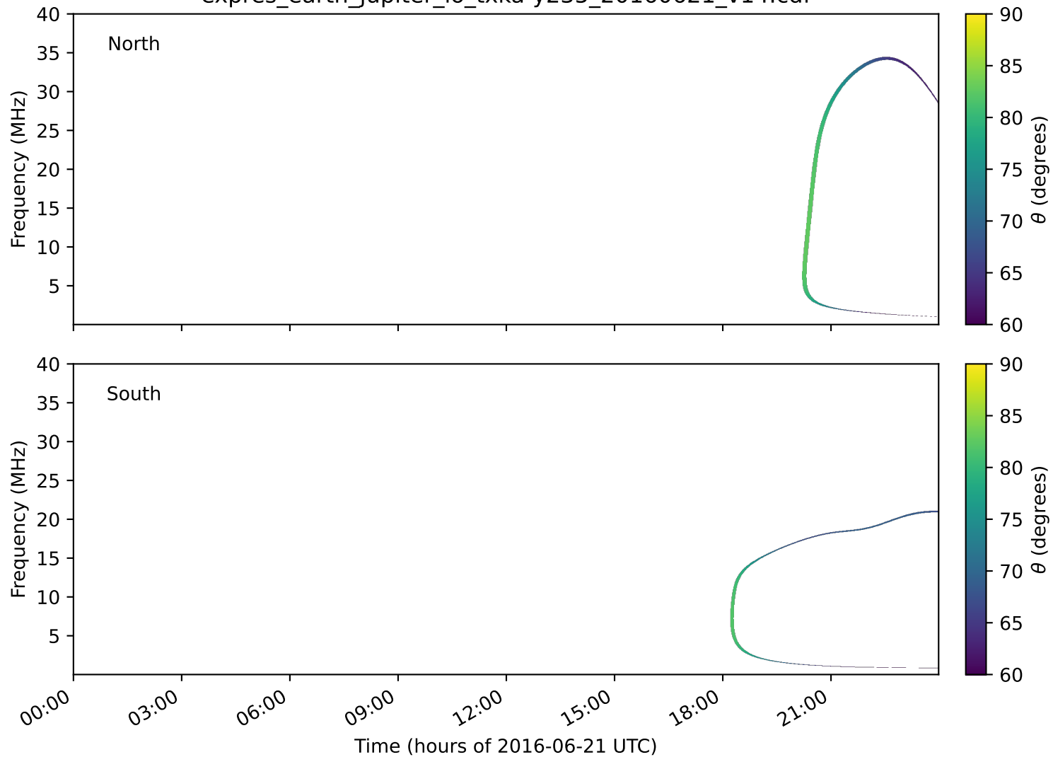
expres_earth_jupiter_io_txka-y235_20160621_v14.cdf
