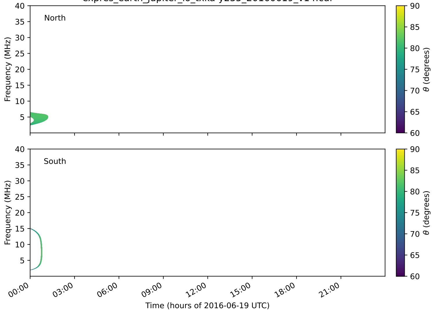
expres_earth_jupiter_io_txka-y235_20160619_v14.cdf
