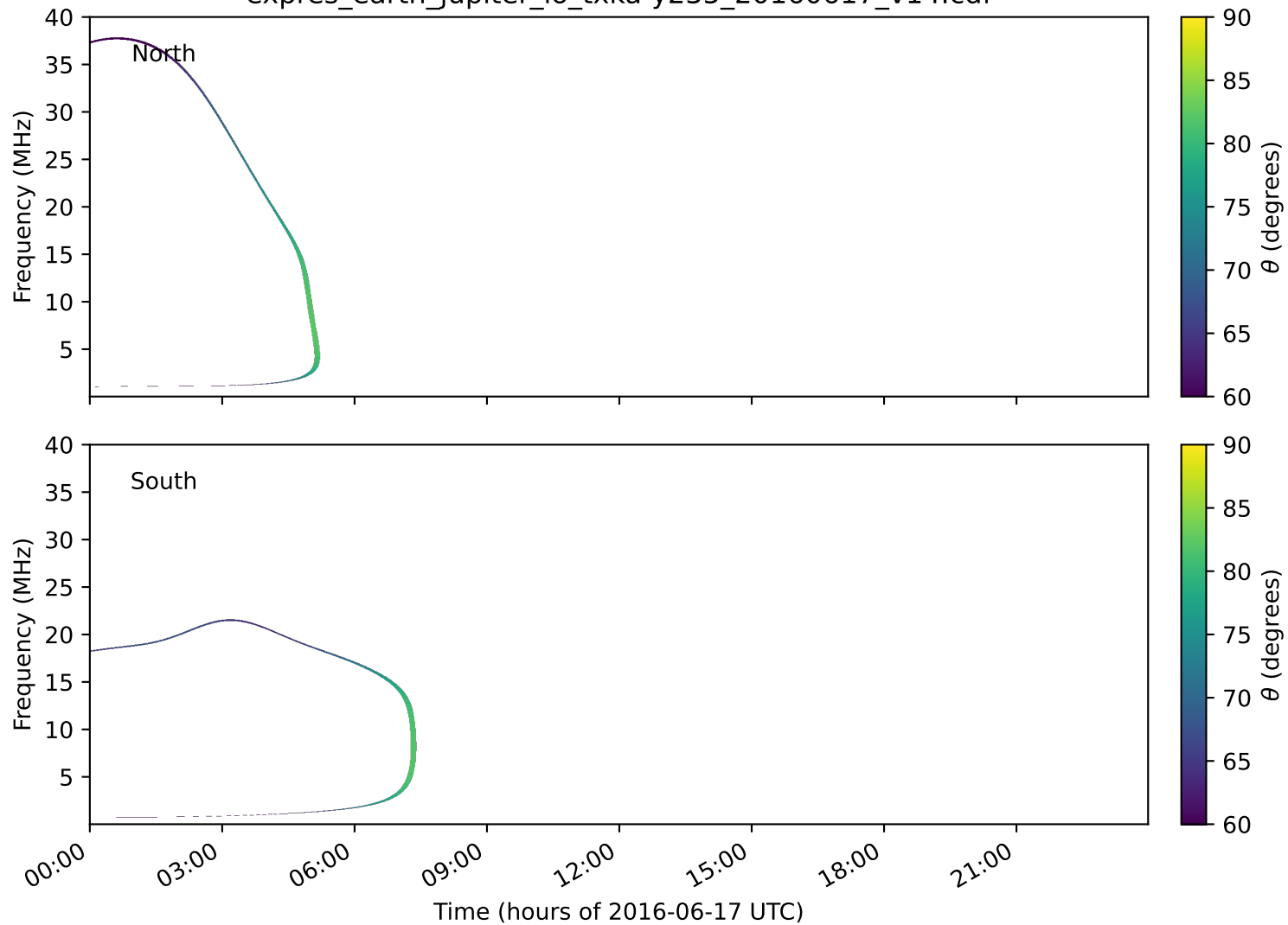
expres_earth_jupiter_io_txka-y235_20160617_v14.cdf
