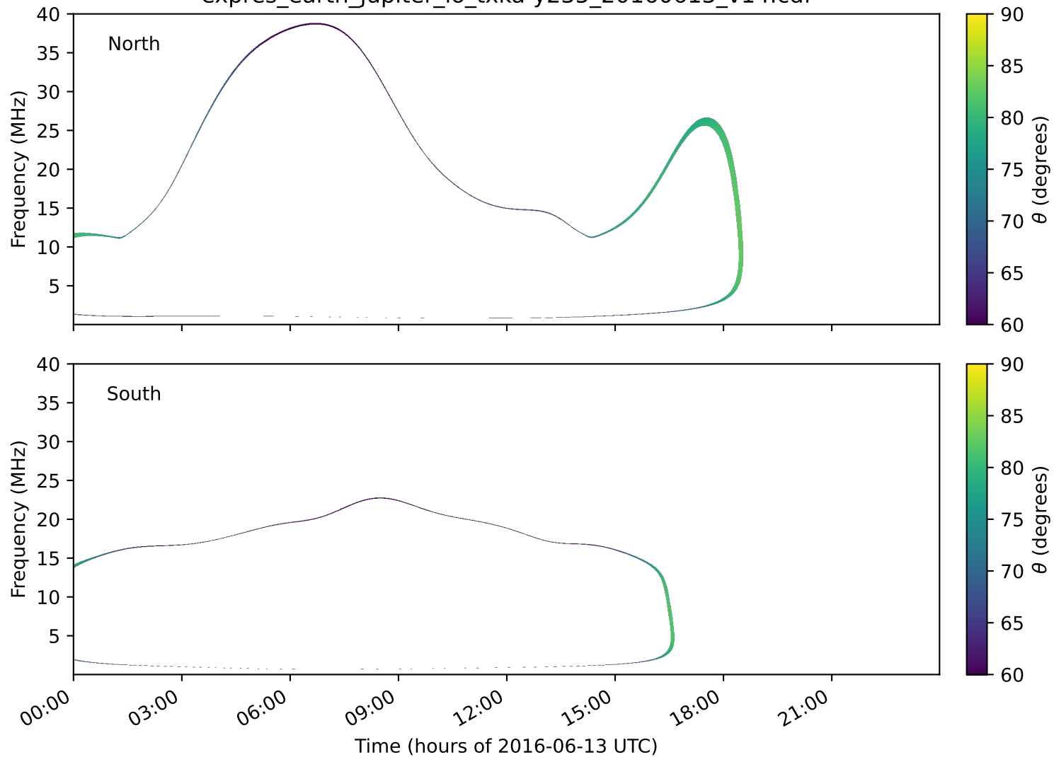
expres_earth_jupiter_io_txka-y235_20160613_v14.cdf
