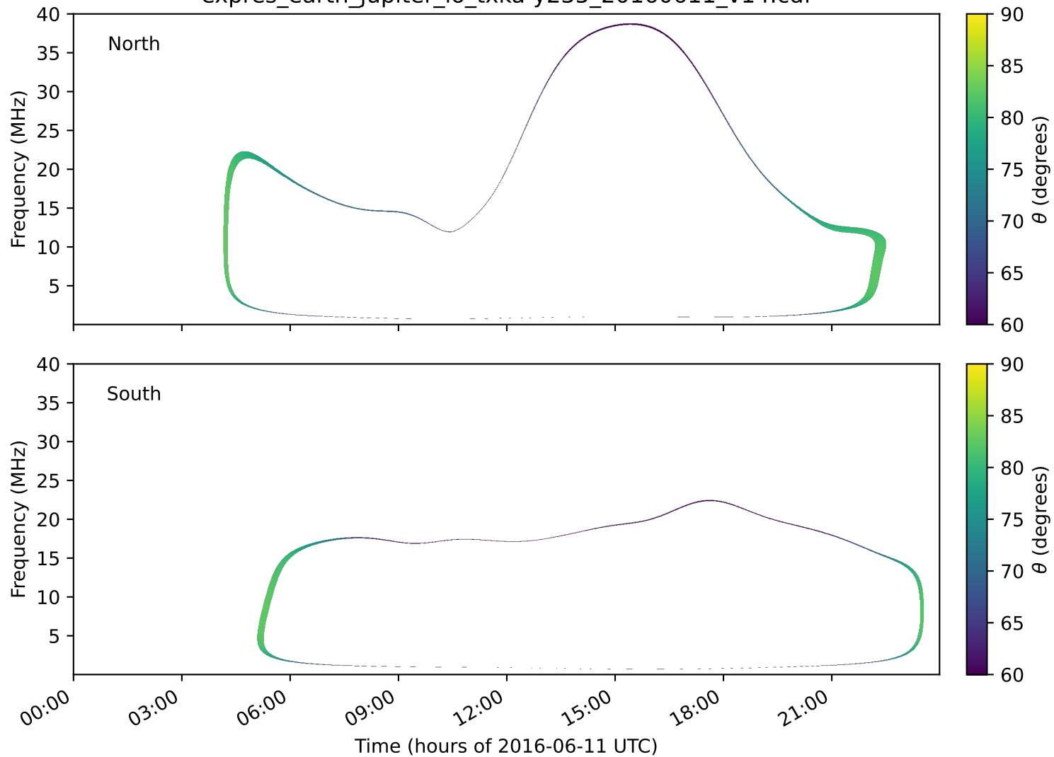
expres_earth_jupiter_io_txka-y235_20160611_v14.cdf
