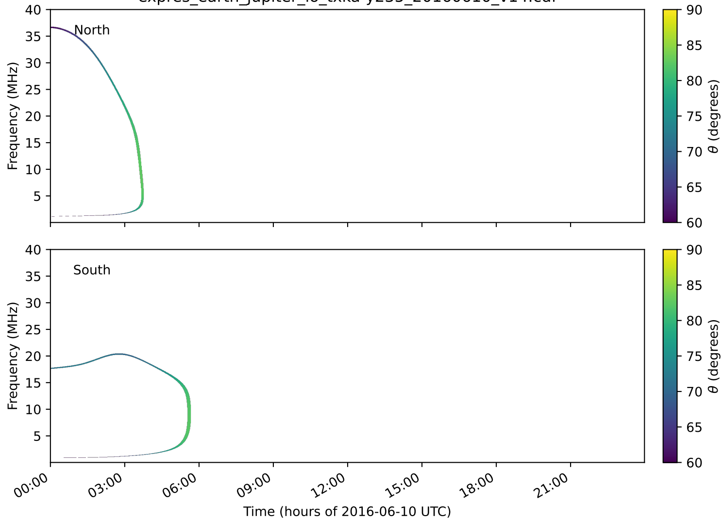
expres_earth_jupiter_io_txka-y235_20160610_v14.cdf
