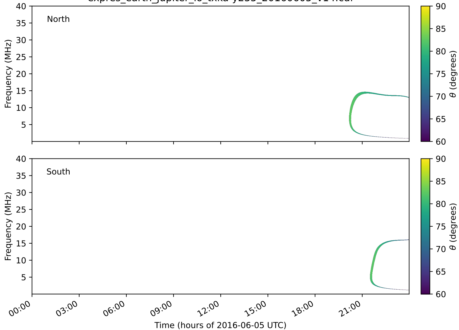
expres_earth_jupiter_io_txka-y235_20160605_v14.cdf
