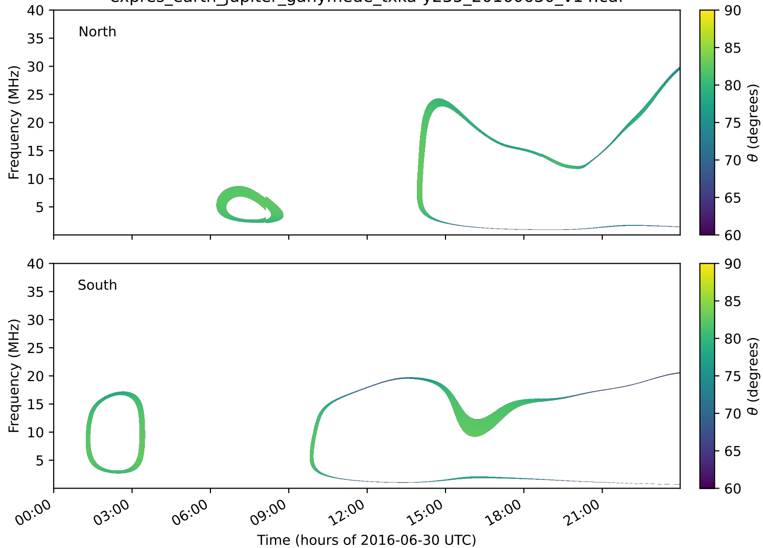
expres_earth_jupiter_ganymede_txka-y235_20160630_v14.cdf
