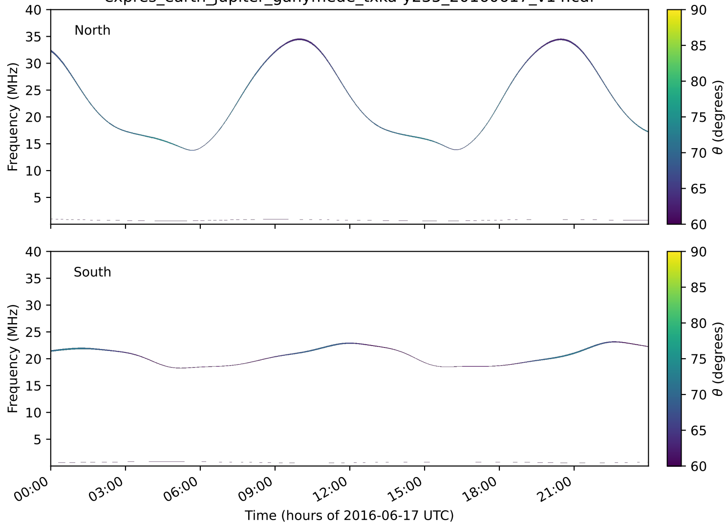
expres_earth_jupiter_ganymede_txka-y235_20160617_v14.cdf
