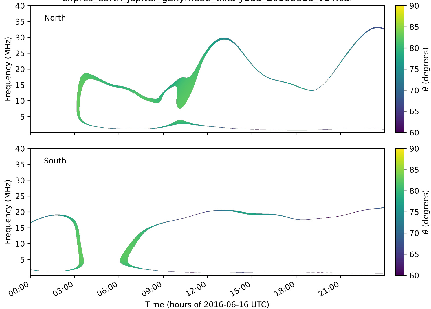
expres_earth_jupiter_ganymede_txka-y235_20160616_v14.cdf
