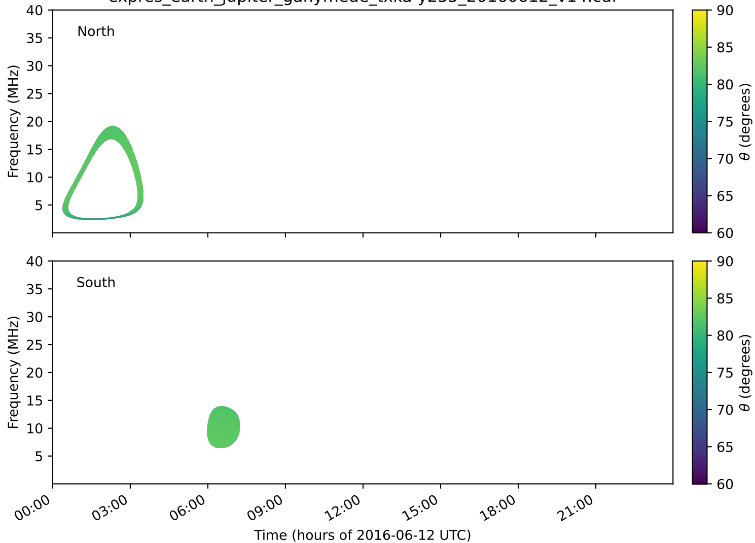
expres_earth_jupiter_ganymede_txka-y235_20160612_v14.cdf
