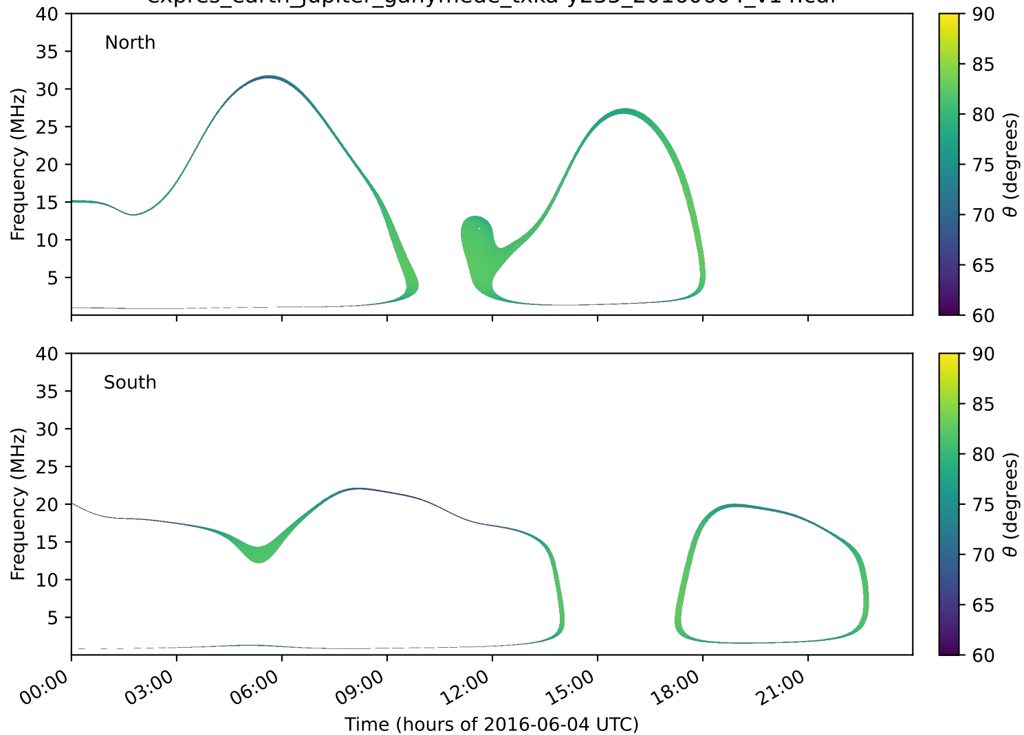
expres_earth_jupiter_ganymede_txka-y235_20160604_v14.cdf
