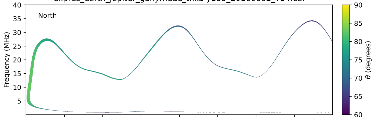
expres_earth_jupiter_ganymede_txka-y235_20160602_v14.cdf
