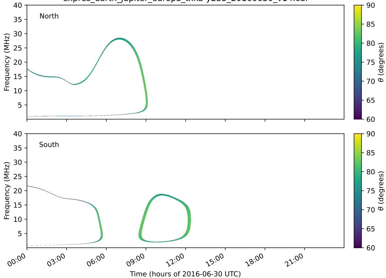
expres_earth_jupiter_europa_txka-y235_20160630_v14.cdf
