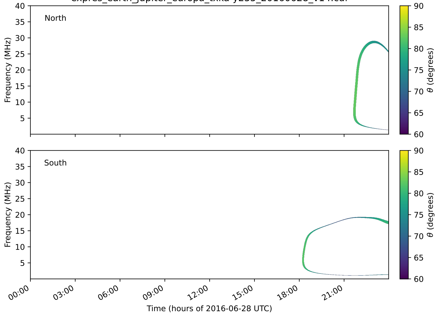
expres_earth_jupiter_europa_txka-y235_20160628_v14.cdf
