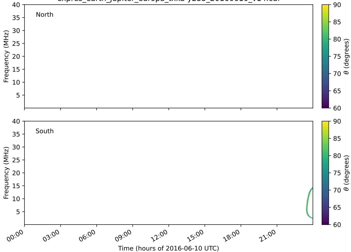
expres_earth_jupiter_europa_txka-y235_20160610_v14.cdf
